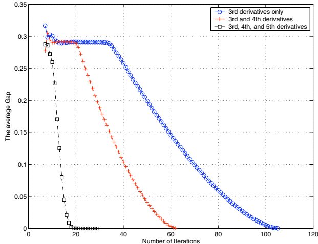
Fig. 2: Gap between original and estimated channel matrix using ALESCAF(3), ALESCAF(3,4), and ALESCAF(3,4,5) for (P, N) = (2, 3) , BPSK sources, infinite block, \theta = \pi/6 .
