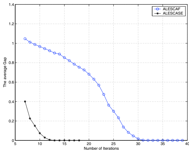
Fig. 3: Gap between original and estimated channel matrix using ALESCAF(6) and ALESCASE for (P, N) = (2, 3) , BPSK sources, infinite block, \theta = \pi/6 .
