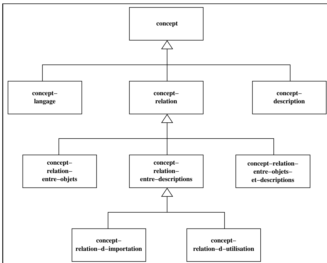
FIG. 5.2 – Les OFL-concepts
