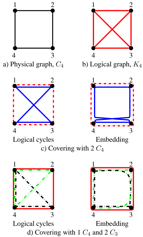
Figure 1: Cycle covering example.
