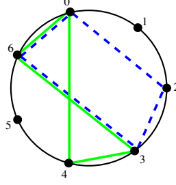
Figure 2: Disjoint Routing Constraint.
