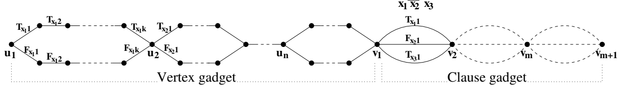
Figure 5: Reduction of MC-Path with colors of span 2 to Maximum 3 Satisfiability
