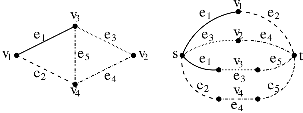
Figure 6: Example of edge-colored graph built from a Max. Independent Set instance.
