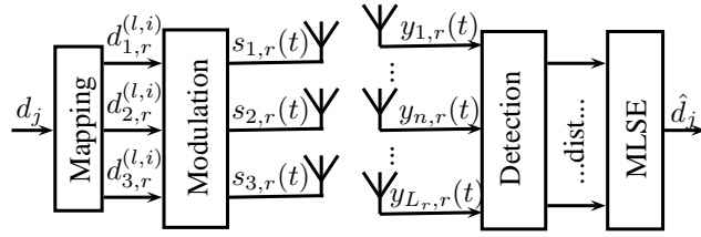
Figure 1: Structure of a MIMO Tx/Rx system
