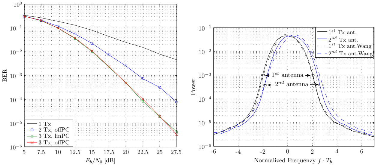
Figure 2: Left: Simulated BER for different numbers of Tx and Rx antennas of the proposed STC and of the Wang-Xia-STC; Right: Simulated psd for each Tx antenna of the proposed STC (continuous line) and the Wang-Xia-STC (dashed line)
