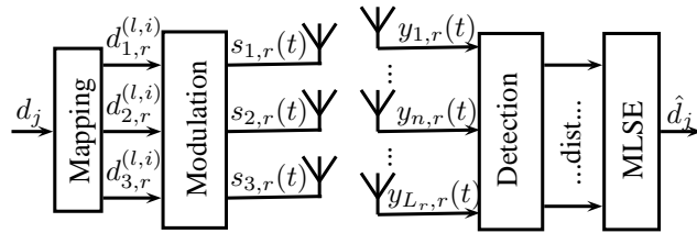
Figure 3: Structure of a MIMO Tx/Rx system
