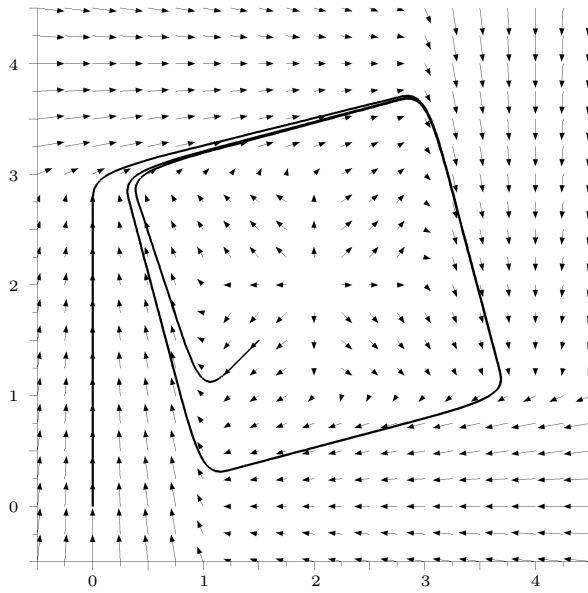
Figure 4: A phase portrait of f with the trajectories starting at (0,0) and (3/2,3/2) . ( \varepsilon = 1/4 , and \varphi_a is defined by \varphi_a(x) = \lambda(x - a) where \lambda is a differentiable increasing function from \mathbb{R} to [0,1] such that \lambda(-\varepsilon) = 0 and \lambda(\varepsilon) = 1 .)
