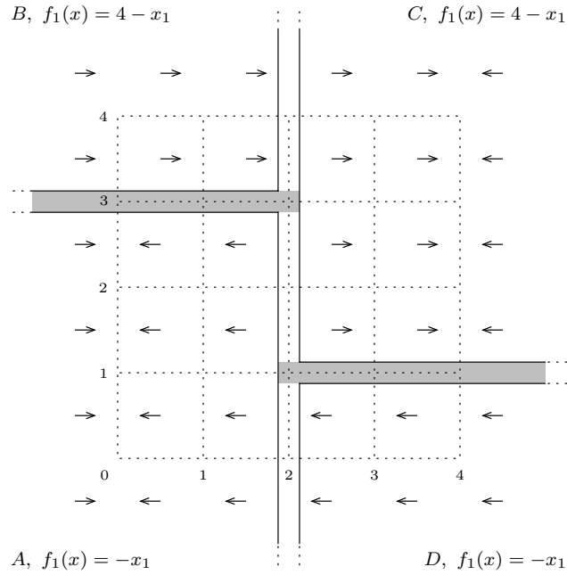
Figure 1: A qualitative phase portrait of f_1 (the arrows represent the sign of df_1/dt and \varepsilon = 1/8 ). It is based on the fact that f_1(x) = -x_1 for x in A = ]-\infty, 2 - \varepsilon[ \times ]-\infty, 3 - \varepsilon] or D = [2 + \varepsilon, +\infty[ \times ]-\infty, 1 - \varepsilon] , and that f_1(x) = 4 - x_1 for x in B = ]-\infty, 2 - \varepsilon] \times [3 + \varepsilon, +\infty[ or C = [2 + \varepsilon, +\infty[ \times [1 + \varepsilon, +\infty[ . The union of the two grey regions corresponds to the set \Lambda_1 considered in the text.
