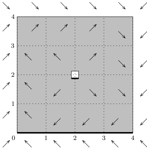
Figure 3: The qualitative phase portrait of f resulting from the qualitative phase portraits of f_1 and f_2 . The grey region corresponds to the set \Omega = [0, 4]^2 \setminus [2 - \varepsilon, 2 + \varepsilon]^2 considered in the text, and the two bold segments correspond to the segments [0, 4] \times \{0\} and [2 - \varepsilon, 2 + \varepsilon] \times \{2 - \varepsilon\} considered in the text.
