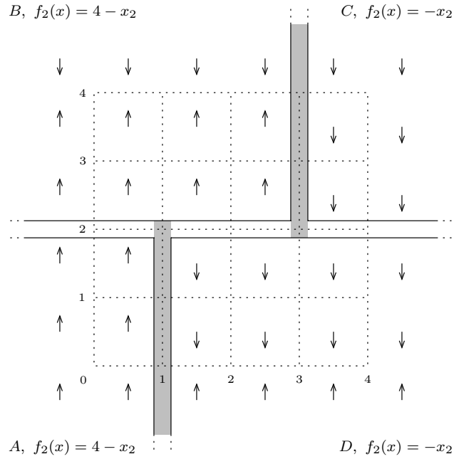
Figure 2: A qualitative phase portrait of f_2 (the arrows represent the sign of df_2/dt and \varepsilon = 1/8 ). It is based on the fact that f_2(x) = 4 - x_2 for x in A = ]-\infty, 1 - \varepsilon] \times ]-\infty, 2 - \varepsilon] or B = ]-\infty, 3 - \varepsilon] \times [2 + \varepsilon, +\infty[ , and that f_2(x) = -x_2 for x in C = [3 + \varepsilon, +\infty[ \times [2 + \varepsilon, +\infty[ or D = [1 + \varepsilon, +\infty[ \times ]-\infty, 2 - \varepsilon] . The union of the two grey regions corresponds to the set \Lambda_2 considered in the text.
