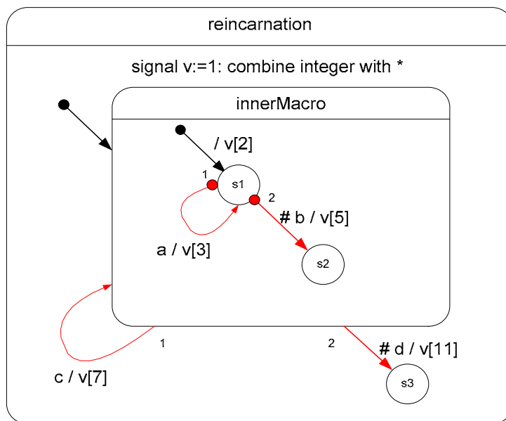
Figure 8-25: Nested Reincarnations.
