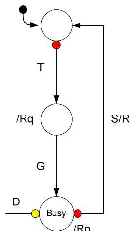
Figure 8-4: Suspension.
