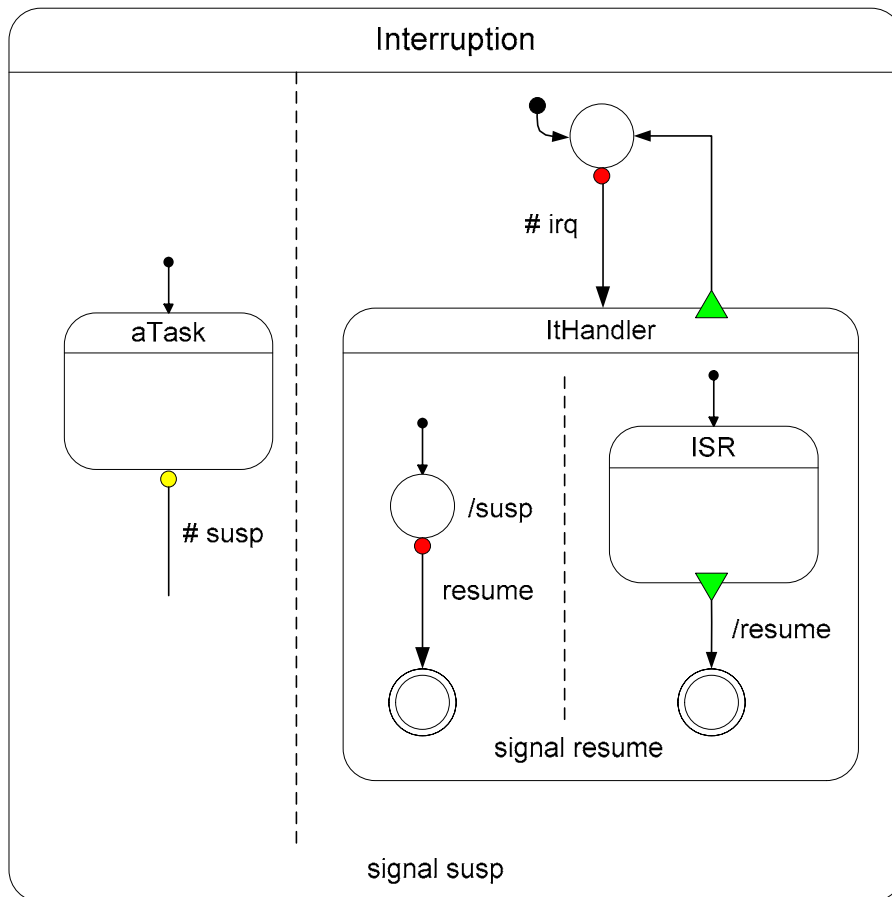
Figure 8-6: Interruption Mechanism.
