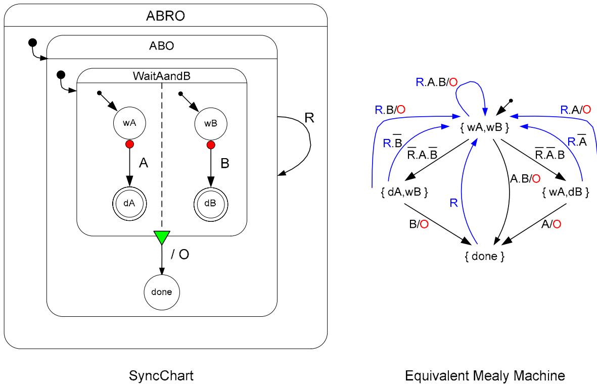
Figure 5-14: SyncChart (variant) for ABRO.
