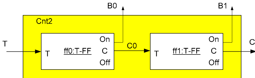
Figure 5-2: A 2-bit binary counter.
