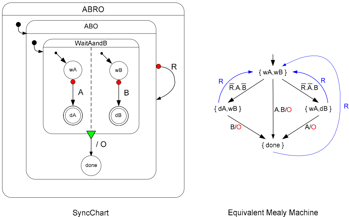
Figure 5-12: SyncChart for ABRO.
