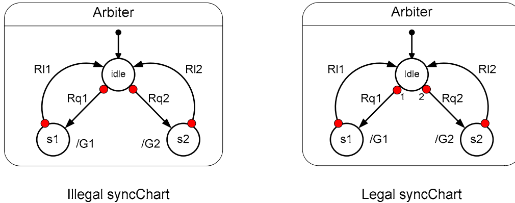
Figure 4-12: SyncChart with Choice.
