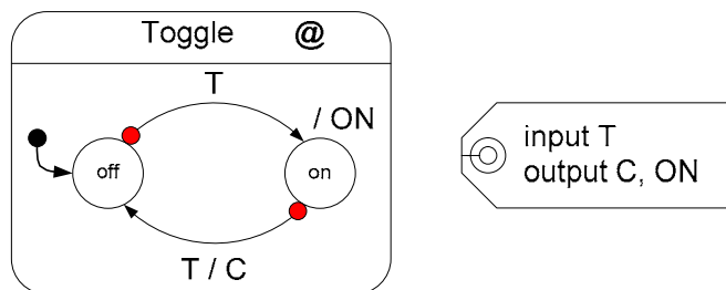
Figure 8-13: SyncChart used as a Reference.
