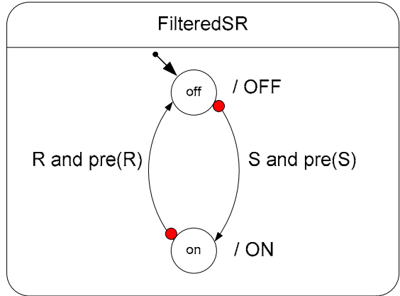
Figure 8-18: Filtered SR Flip-Flop.
