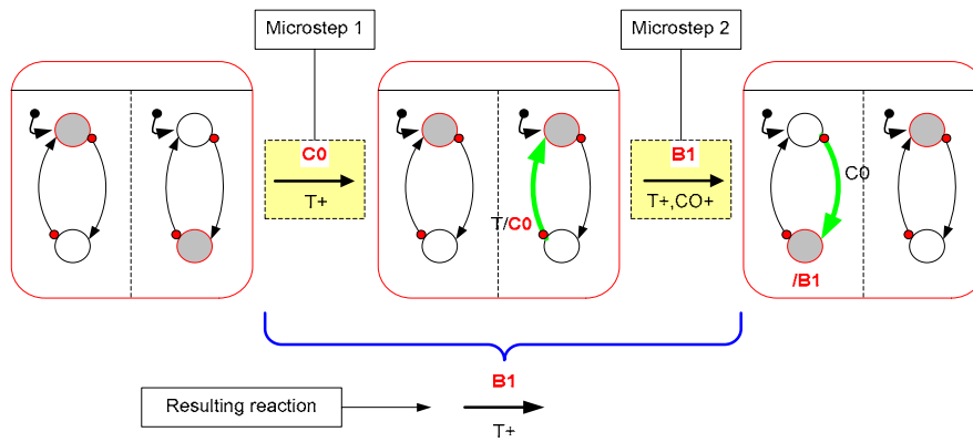
Figure 5-5: Microsteps.
