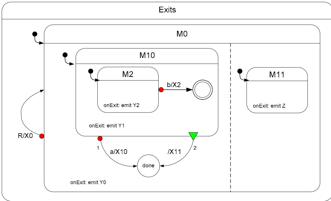
Figure 8-8: Exit Actions.
