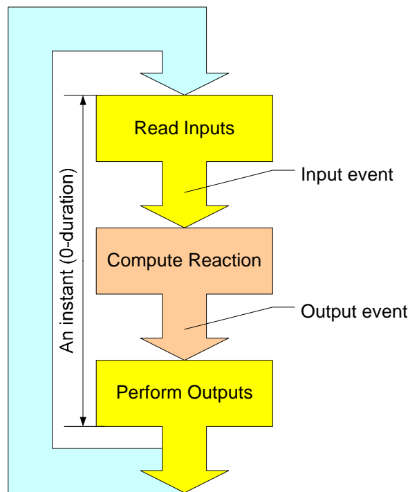
Figure 4-2: Cyclic evolution.
