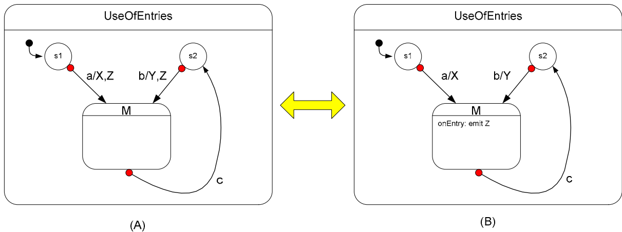
Figure 8-7: Entry Actions.
