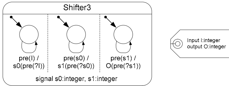
Figure 8-19: Shift Register.
