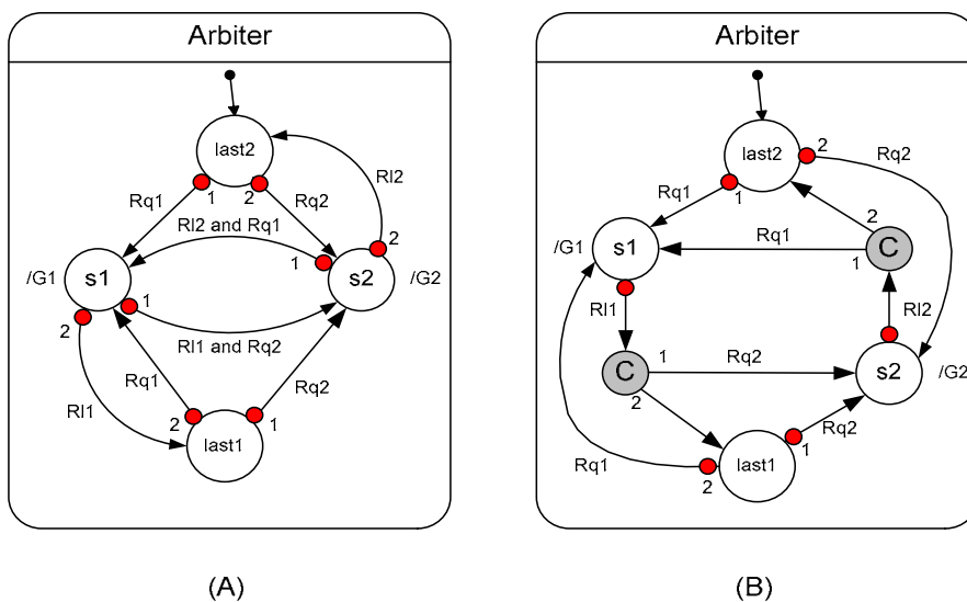
Figure 8-21: Arbiter with Turning Priority.
