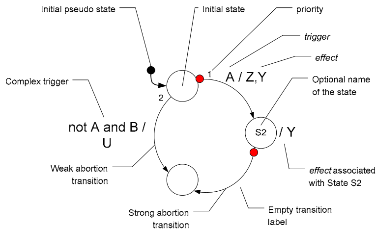
Figure 4-14: FSM notations
