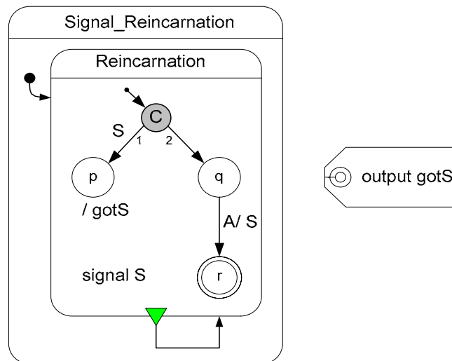
Figure 8-22: Signal Reincarnation.
