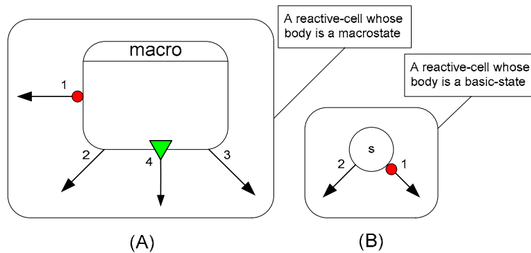
Figure 6-2: Reactive Cells.
