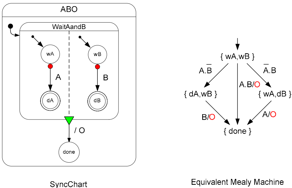
Figure 5-9: Synchronized Termination.
