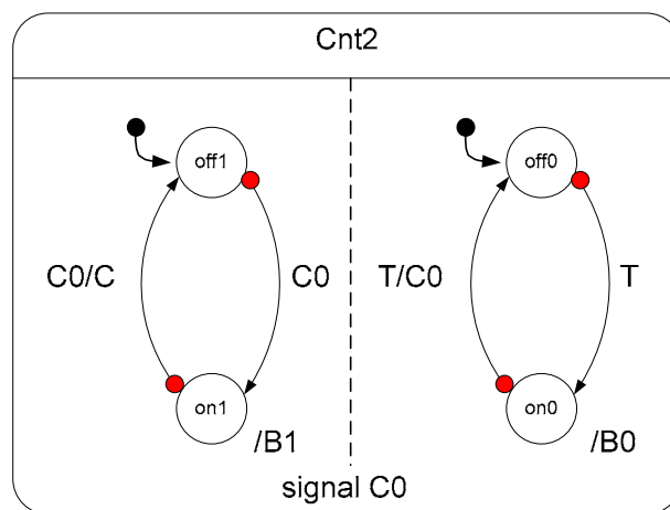
Figure 5-3: SyncChart for a 2-bit binary counter.
