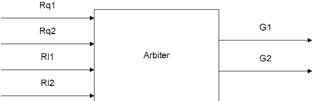
Figure 10-7: Interface of Arbiter.
