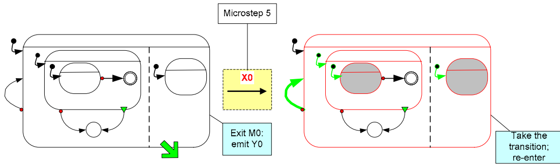
Figure 8-11: Microsteps of a reaction with exit actions (3).
