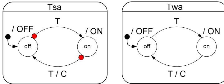
Figure 4-5: SyncCharts for the Toggle Flip-Flop—Strong and weak abortion versions.
