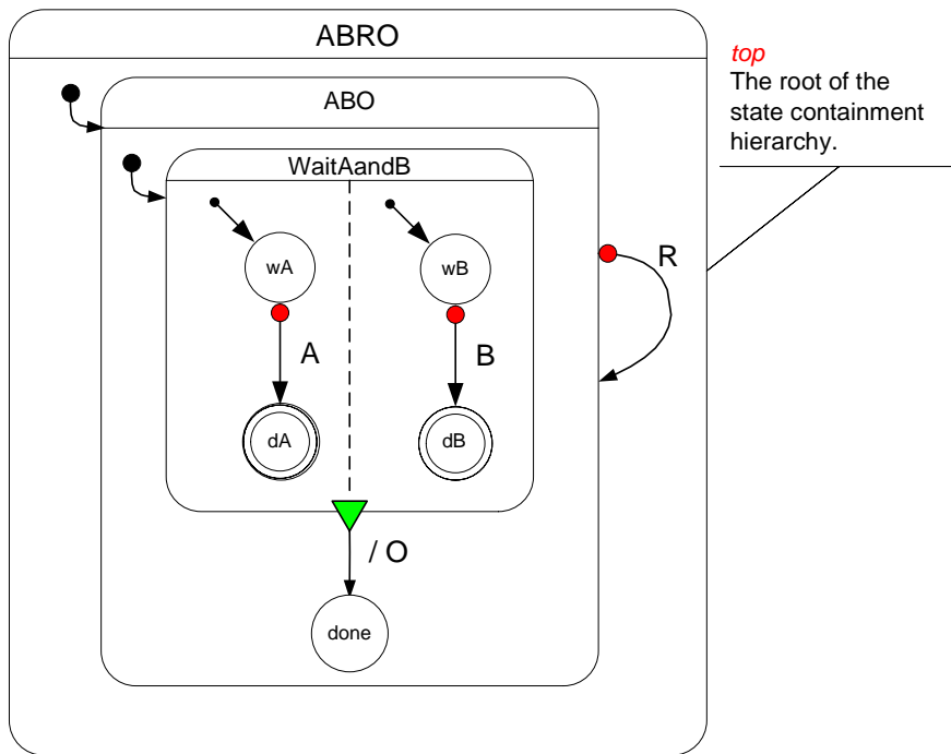
Figure 6-1: A SyncChart.
